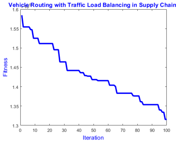
Fig. 4. The optimization process of the PSO algorithm proposed by the research
