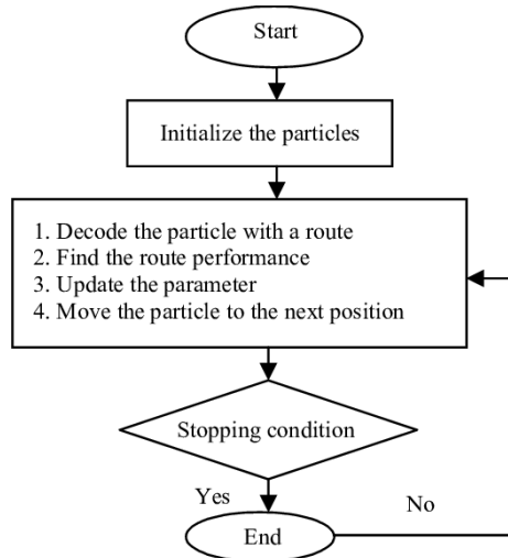
Fig. 2. Flowchart of the proposed PSO routing method of vehicles in the supply chain
